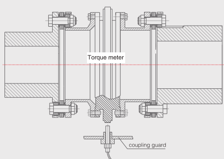
d.with torque measure
