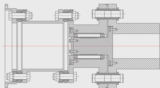
c.design of overload protection
